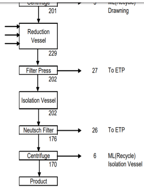
DASDA MASS BALANCE OF DASDA
